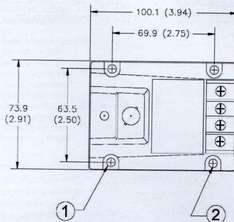
Figure 1: 990 Vibration Transmitter Dimensions (top view)
